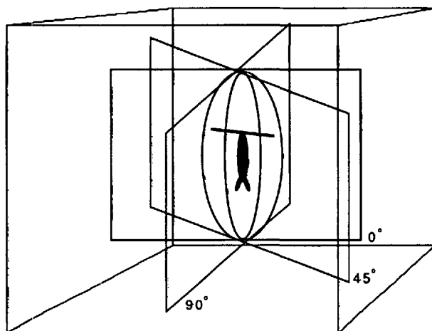
Figure 1. Three planes in which particle trajectories for Pleuromamma xiphias were mapped.
