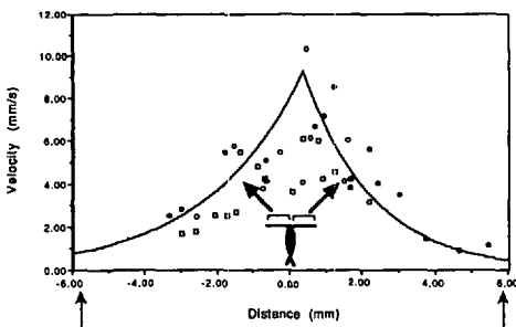
Figure 4 (left). Profile of the water velocity along the first antennae of Pleuromamma xiphias . Increasing negative values represent distance traveled toward the distal tip along the left antennae while positive values are the distances traveled along the right antennae. Symbols represent data taken from three different animals. The curve is an exponential fit to data derived from contour. Arrows indicate distal tips of the antennae.
