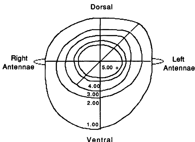
Figure 6. Water velocity through the antennal plane. A cross section of the flow field of Pleuromamma xiphias defined by the plane perpendicular to the body of the animal encompassing the first antennae. Values shown are in units of \text{mm} \cdot \text{s}^{-1} .
