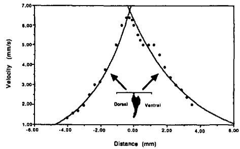
Figure 4 (left). Profile of the water velocity along the first antennae of Pleuromamma xiphias . Increasing negative values represent distance traveled toward the distal tip along the left antennae while positive values are the distances traveled along the right antennae. Symbols represent data taken from three different animals. The curve is an exponential fit to data derived from contour. Arrows indicate distal tips of the antennae.
