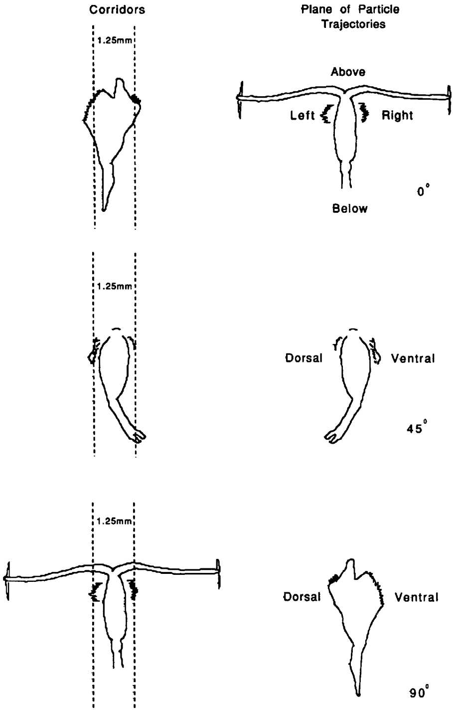
Figure 2. Corridors used in the analysis of the velocity isopleths and particle trajectories for the dorsal view (A), 45 degree view (B) and lateral view (C) of Pleuromamma xiphias .
