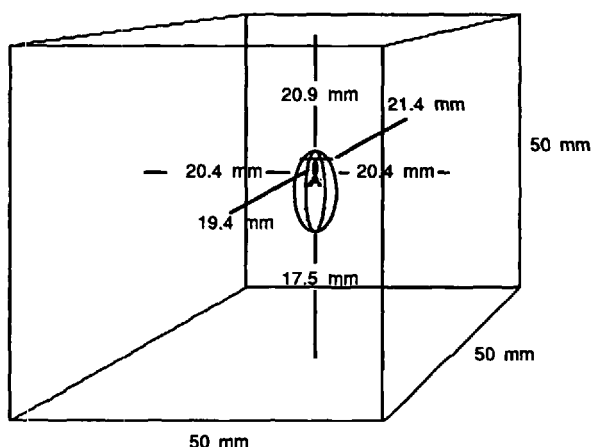
Figure 7. Dimensions of flow field. The dimensions of the flow field defined by the 1.00-mm isopleth with respect to the size of the filming container.
