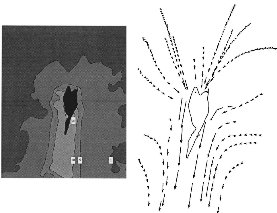
Figure 3E. Velocity isopleths—lateral view. Legend same as Figure 3A. Figure 3F. Particle trajectories—lateral view. Legend the same as Figure 3A.
